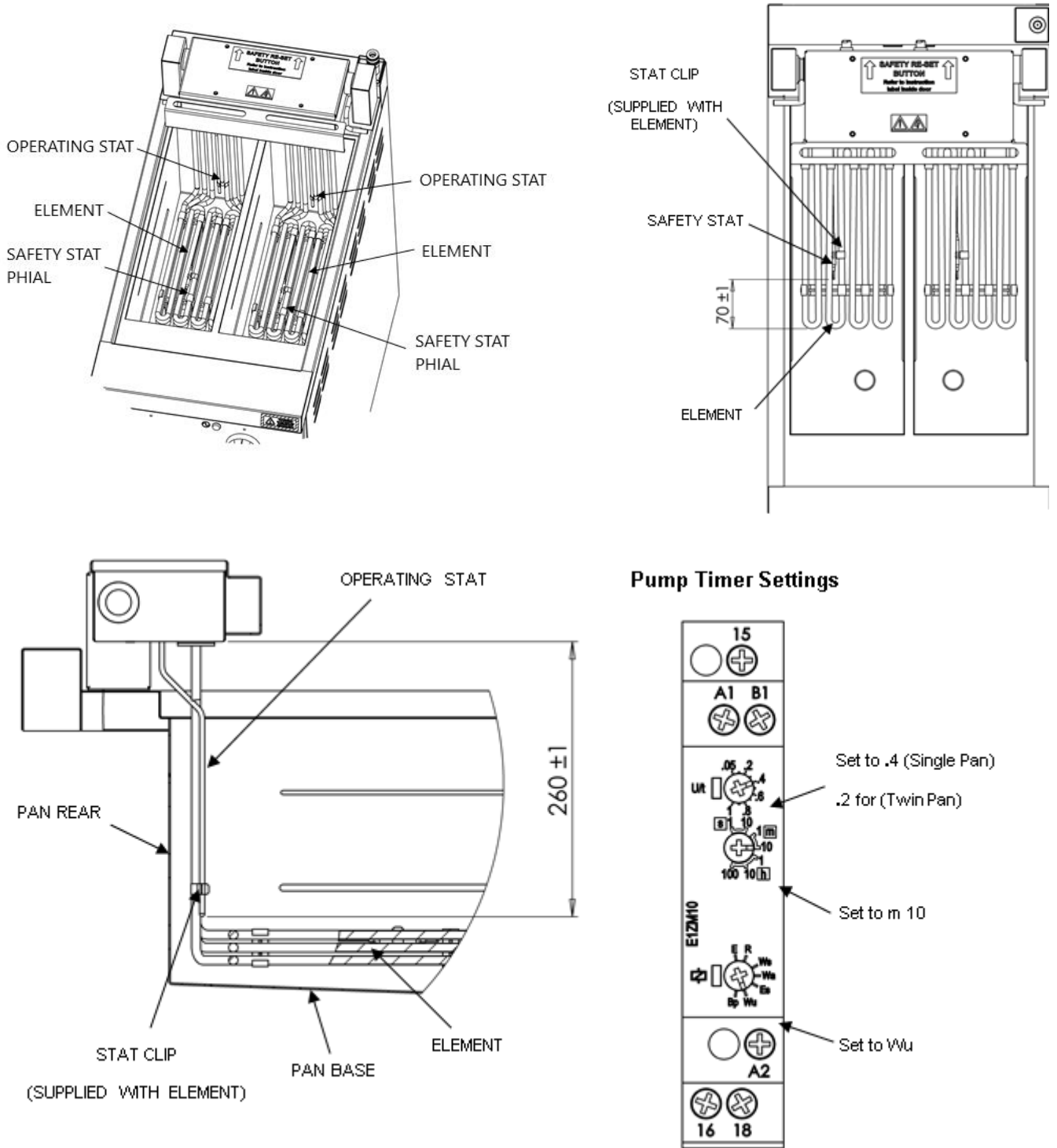
Figure 9 – Critical dimensions
